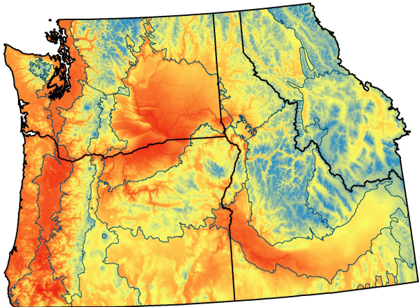
1986 - 2010 Mean Annual Temperature (°C)
