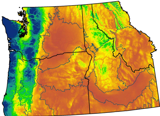
1986 - 2010 Mean Annual Precipitation (mm)
