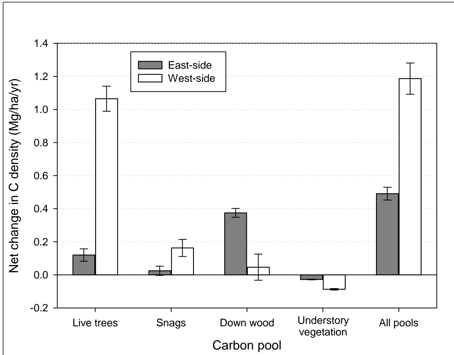
Fig. A.2. Estimated mean and standard error of C stock flux components for west-side and east-side PNW national forest lands, 1995-2002.
